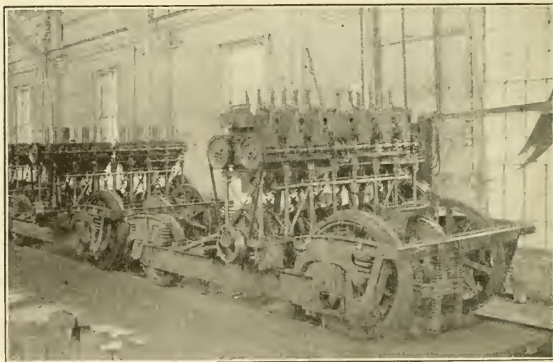
Fig. 11. Front Trucks of McKean Gasoline Motor Car Assembled with Engine.
